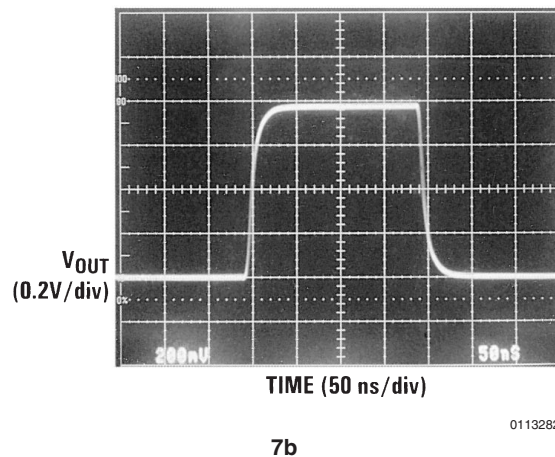
FIGURE 7. RC Limits Amplifier Bandwidth to 50 MHz, Eliminating Peaking in the Resulting Pulse Response
