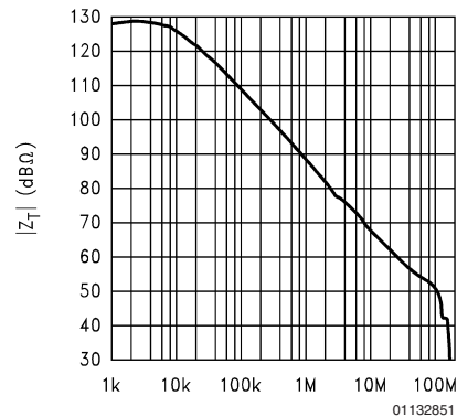
TRANSIMPEDANCE vs FREQUENCY V_S = \pm 15\text{V} R_L = 1k\Omega
