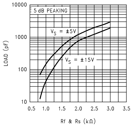
SUGGESTED R_f and R_S FOR C_L A_V = -1
