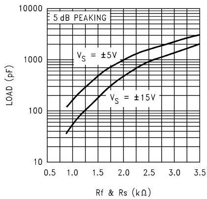
SUGGESTED R_f and R_S FOR C_L A_V = +2
