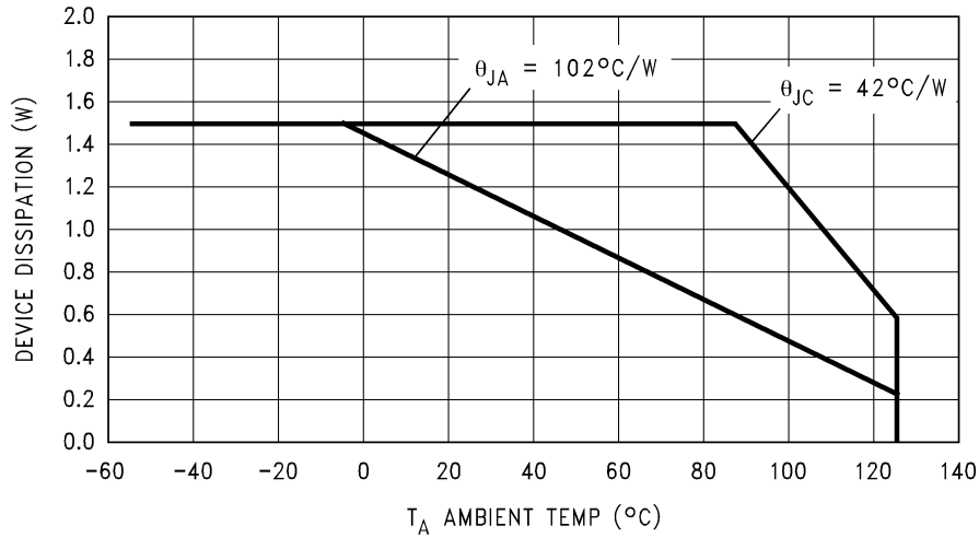
N-Package
