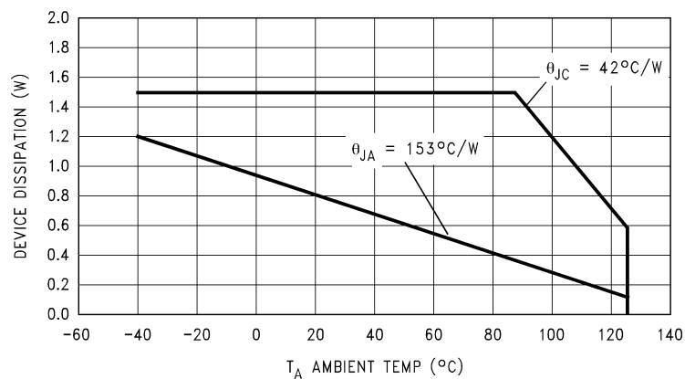
M-8 Package
