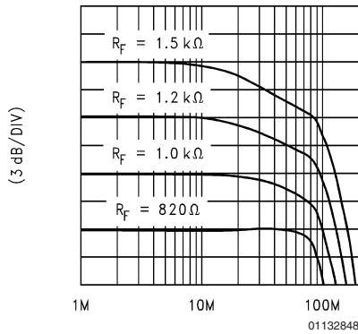
NON-INVERTING GAIN FREQUENCY COMPENSATION V_S = \pm 15\text{V} ; A_V = +2 ; R_L = 150\Omega
