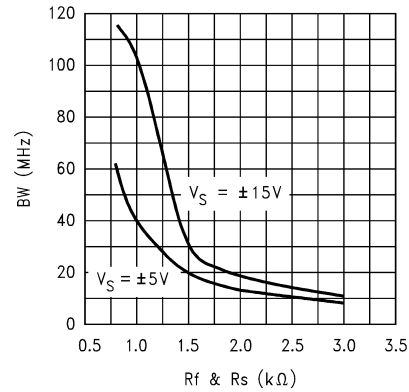
BANDWIDTH vs R_f & R_S A_V = -1 , R_L = 1k\Omega
