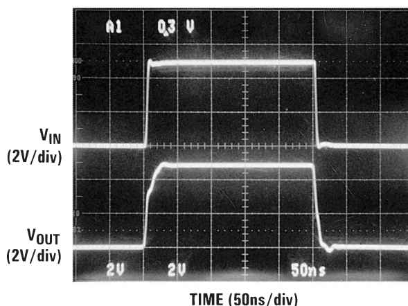
Cable Driver
