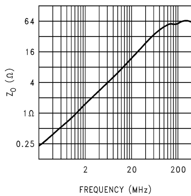
OUTPUT IMPEDANCE vs FREQ V_S = \pm 5\text{V} ; A_V = -1 R_f = 820\Omega
