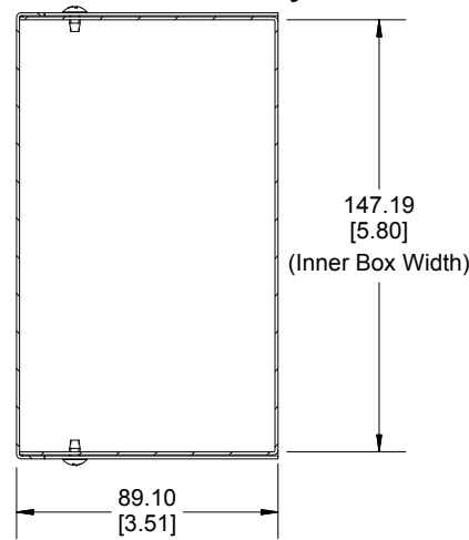
SECTION A-A End View of Assembly
