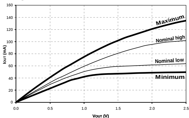
Figure 7: Pull-Down Characteristics
