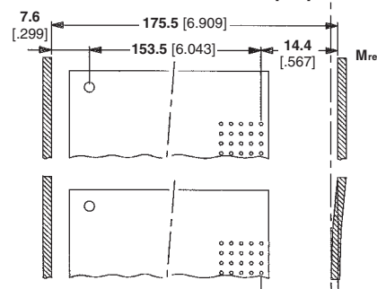
Subrack tolerances
