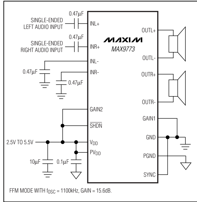
Figure 7. Single-Ended Input
