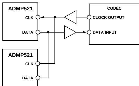
Figure 13. Buffered Connection Between Stereo ADMP521s and a Codec
