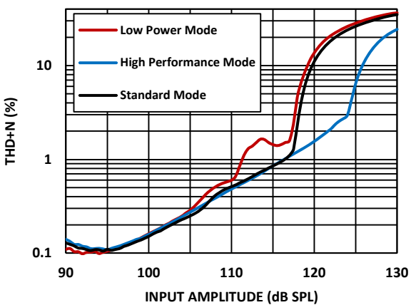
Figure 5. THD + N vs. Input Level
