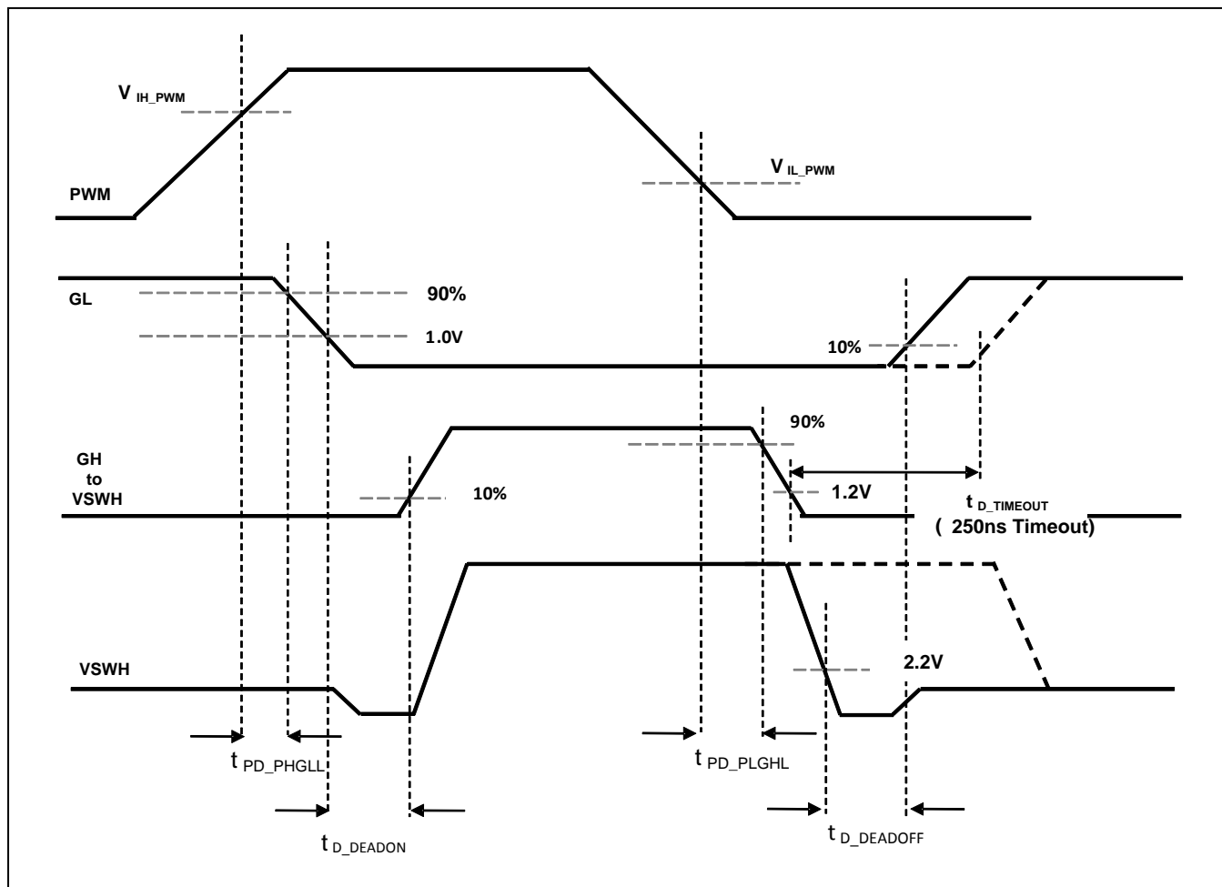
Figure 2.6 PWM Timing
