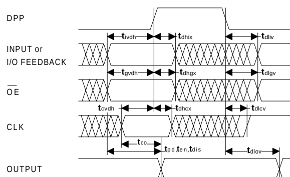
Figure 3. DPP Timing Waveform
