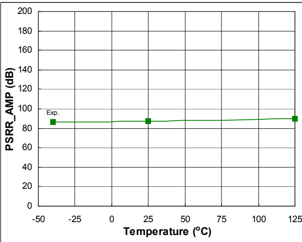
Fig. 70. Operational Amplifier Power Supply Rejection Ratio vs. Temperature
