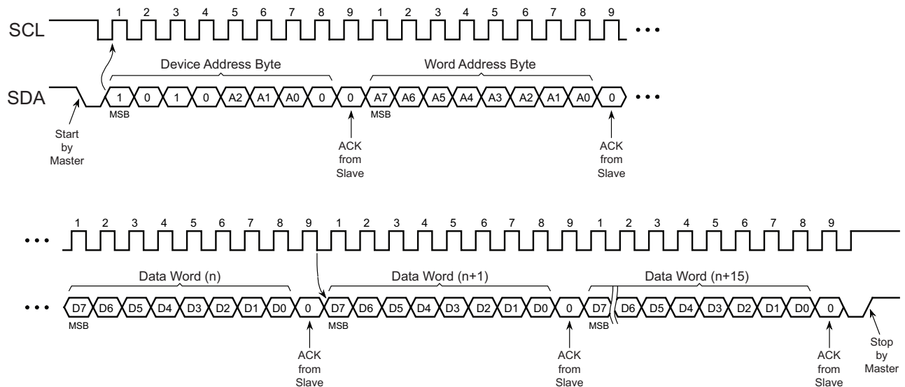
Figure 6-7. Page Write
