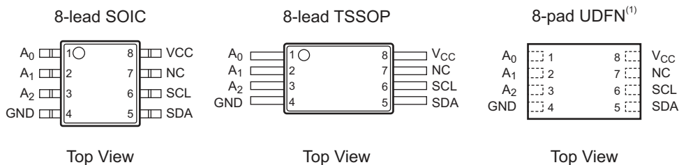
Figure 1-1. Pinouts
