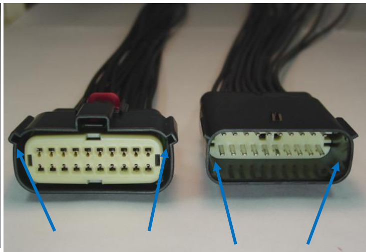
Keying Features
