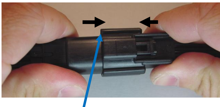
Primary Latch
