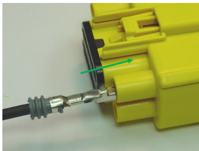
Note alignment tabs on Receptacle terminal
