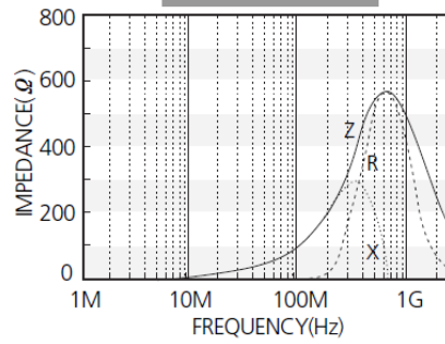
CIM03U121
