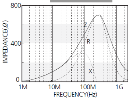
CIM03U471
