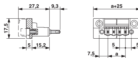
Dimensioned drawing
