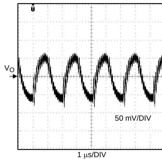
Figure 9. Output Voltage Ripple AC Coupled ( V_{IN} = 24V , I_O = 0.5A )
