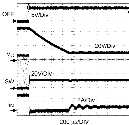
Figure 13. Shutdown ( V_{IN} = 12V , I_O = 0.5A )
