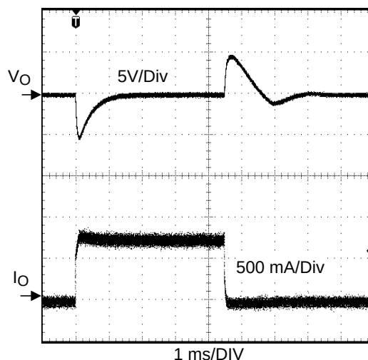
Figure 11. Load Transient Response ( V_{IN} = 24V , I_O = 0 to 0.7A )
