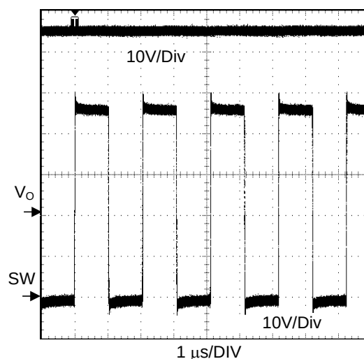
Figure 7. Switch Node Voltage ( V_{IN} = 24V , I_O = 0.5A )
