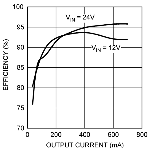
Figure 2. Efficiency
