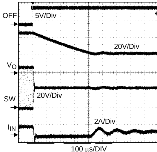
Figure 15. Shutdown ( V_{IN} = 24V , I_O = 0.5A )
