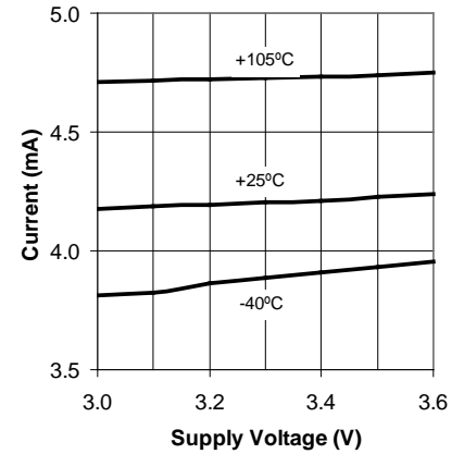
Current vs. Supply Voltage f_{RF} = 315MHz
