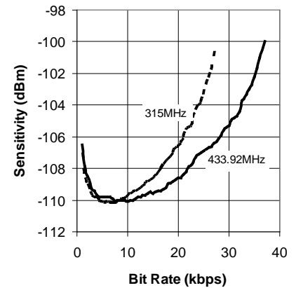
Sensitivity at 1% BER V_{SEL1} = 3.3V, V_{SEL0} = 0V
