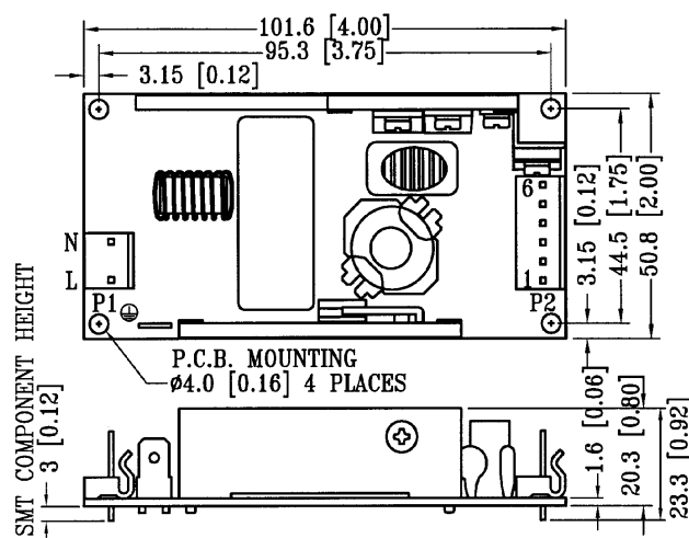
TRIPLE OUTPUT
