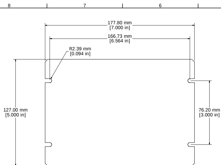
1431-12 OR 1431-12BK3 - VIEW FROM TOP (SOLD SEPERATELY)
