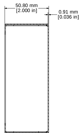
SECTION EE-EE
