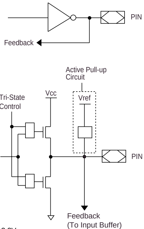
Typical Output
