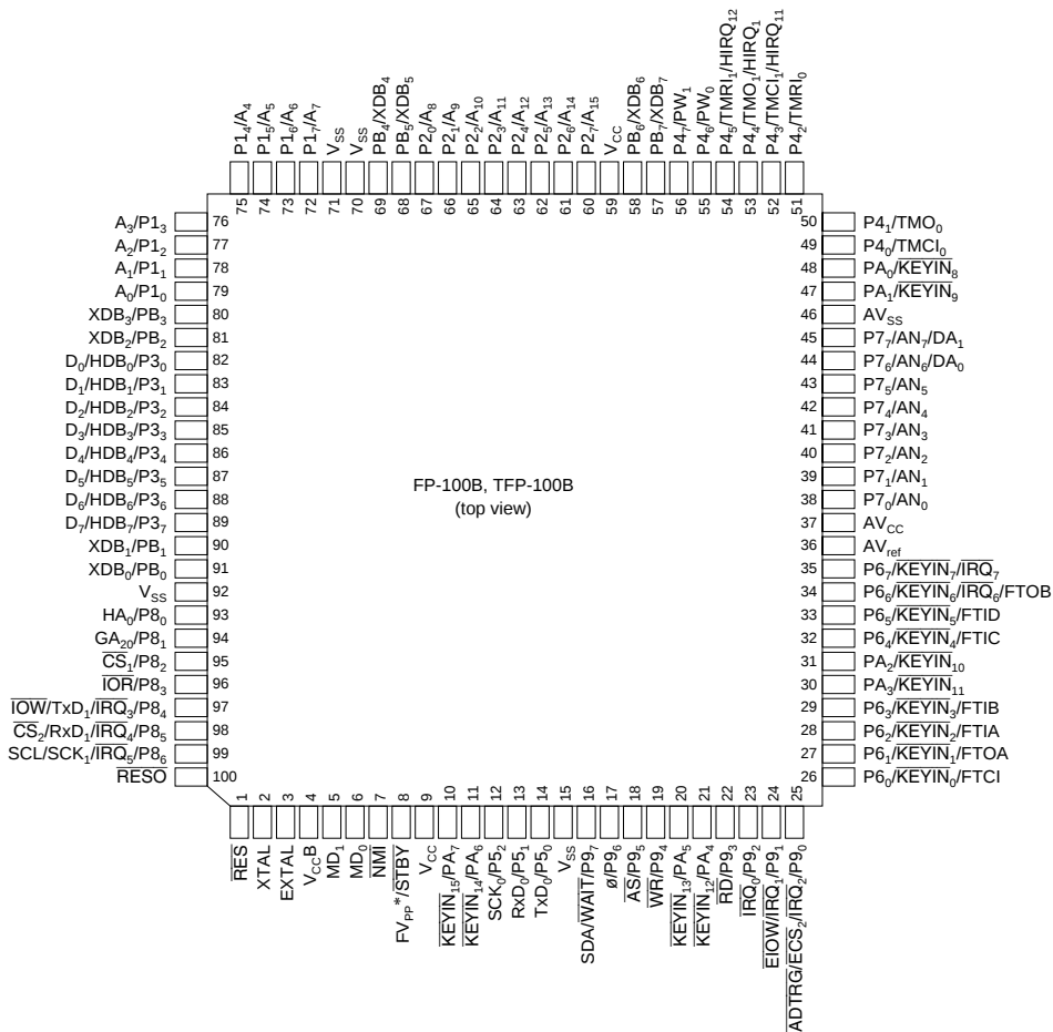
Figure 1.2 Pin Arrangement (FP-100B, TFP-100B, Top View)
