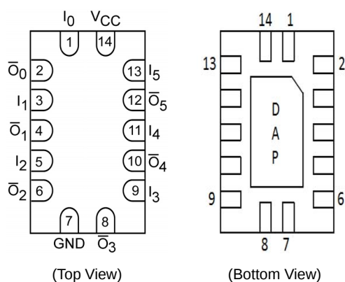
Figure 2. Pin Assignment for DQFN
