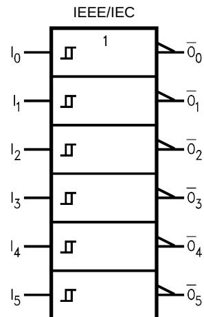
Figure 3. Logic Symbol
