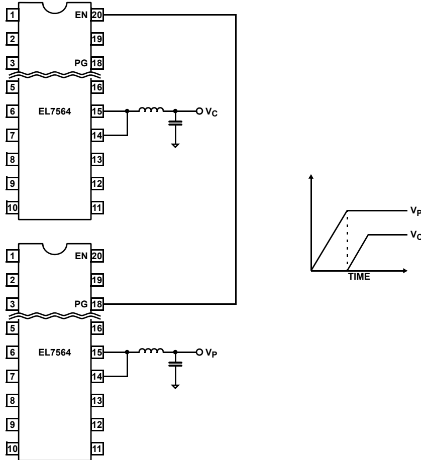
FIGURE 26. OFFSET TRACKING
