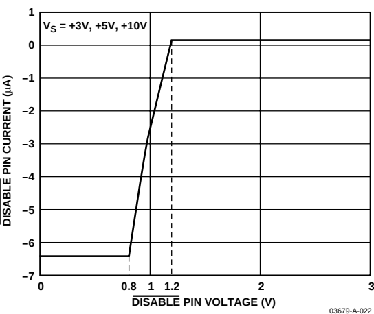
Figure 49. AD8029 \overline{\text{DISABLE}} Pin Current vs. \overline{\text{DISABLE}} Pin Voltage
