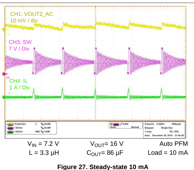
Figure 27. Steady-state 10 mA
