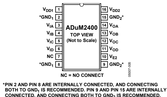
Figure 5. ADuM2400 Pin Configuration
