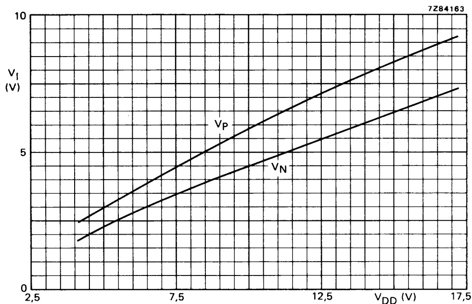
Fig. 9 Typical switching levels as a function of supply voltage V_{DD} ; T_{amb} = 25^{\circ}C .
