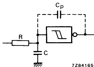
Fig. 10 Schmitt trigger driven via a high impedance ( R > 1\text{ k}\Omega ).
