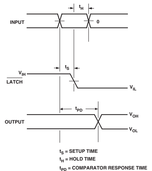
Figure 4. Latch Timing
