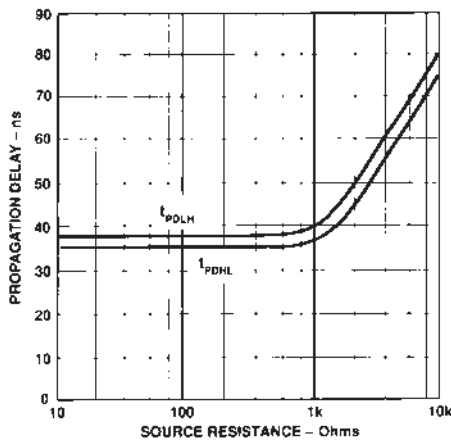
TPC 4. Propagation Delay vs. Source Resistance
