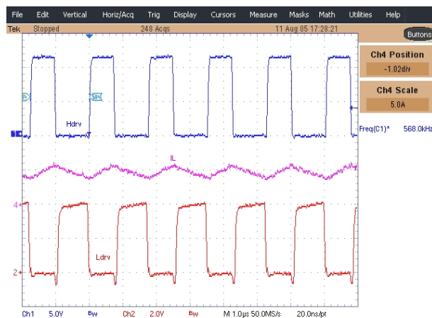
Figure 16 - Gates waveforms Ch1:Hdrv, Ch2:Ldrv, Ch4:Inductor Current I_{Load}=5A
