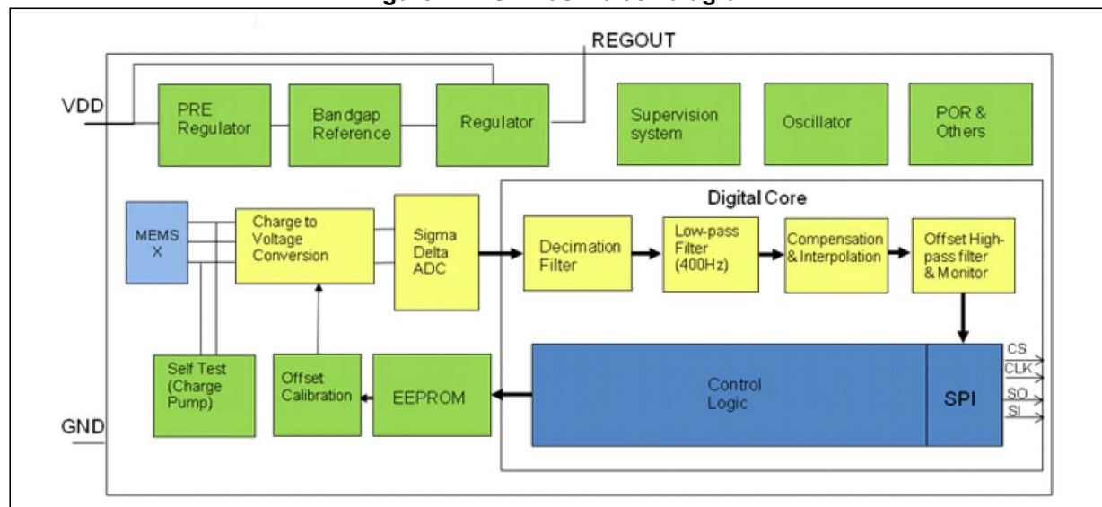
Figure 1. AIS1120SX block diagram
