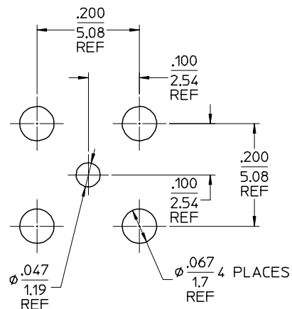
RECOMMENDED BOARD LAYOUT
