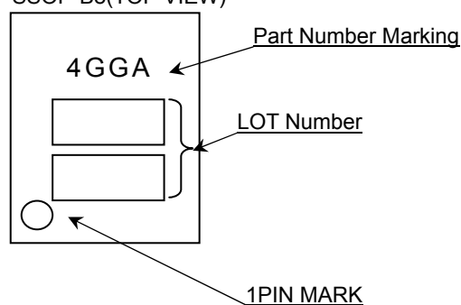
SSOP-B8(TOP VIEW)
