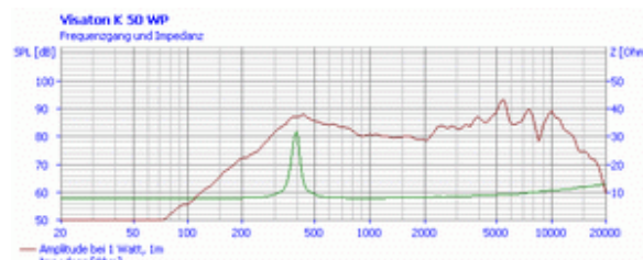
frequency- and impedance response
