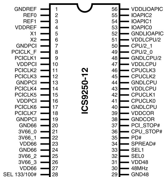
56-pin SSOP
