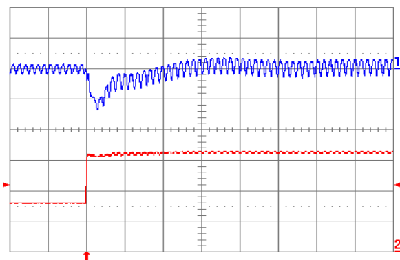
Fig. 3.3V.7: Output voltage response for V_{out} = 3.3 V to positive load current step change from 2.5 A to 5 A with slew rate of 5 A/ \mu s at V_{in} = 5 V. Top trace: output voltage (100 mV/div.); Bottom trace: load current (2 A/div.). C_o = 47 \mu F ceramic + 1 \mu F ceramic. Time scale: 20 \mu s/div.
