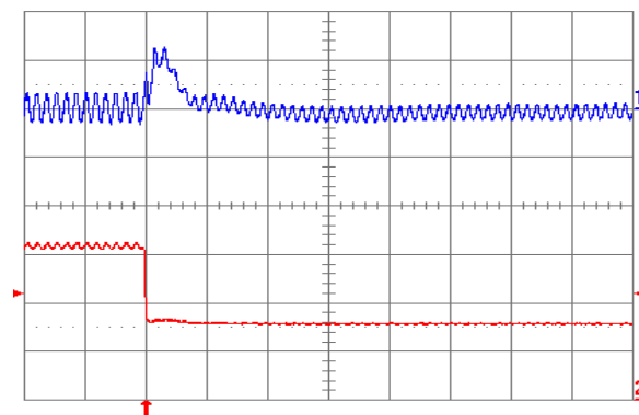
Fig. 2.0V.8: Output voltage response for V_{out} = 2.0 V to negative load current step change from 5 A to 2.5 A with slew rate of -5 A/ \mu s at V_{in} = 5 V. Top trace: output voltage (100 mV/div.); Bottom trace: load current (2 A/div.). C_o = 47 \mu F ceramic + 1 \mu F ceramic. Time scale: 20 \mu s/div.
