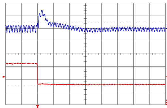
Fig. 3.3V.8: Output voltage response for V_{out} = 3.3 V to negative load current step change from 5 A to 2.5 A with slew rate of -5 A/ \mu s at V_{in} = 5 V. Top trace: output voltage (100 mV/div.); Bottom trace: load current (2 A/div.). C_o = 47 \mu F ceramic + 1 \mu F ceramic. Time scale: 20 \mu s/div.
