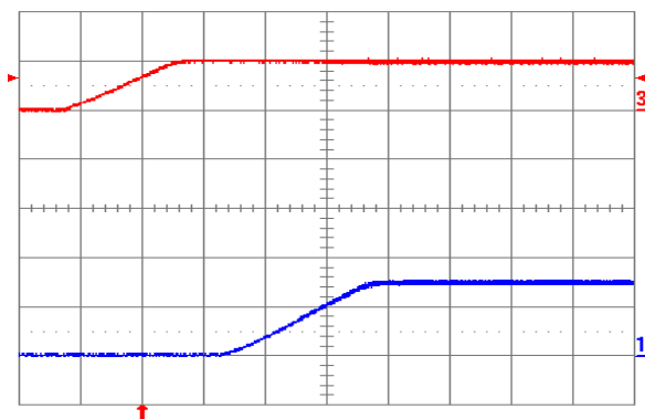
Fig. 1.5V.5: Turn-on transient for V_{out} = 1.5 V with application of V_{in} at full rated load current (resistive) and 47 \mu F external capacitance at V_{in} = 5 V. Top trace: V_{in} (5 V/div.); Bottom trace: output voltage (1 V/div.); Time scale: 2 ms/div.
