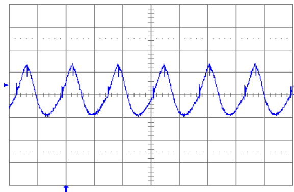
Fig. 1.0V.6: Output voltage ripple (20 mV/div.) at full rated load current into a resistive load with external capacitance 10 \mu F ceramic + 1 \mu F ceramic and V_{in} = 5 V for V_{out} = 1.0 V. Time scale: 2 \mu s/div.
