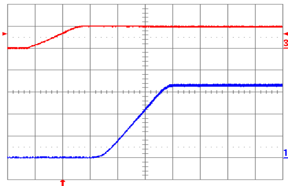
Fig. 3.3V.5: Turn-on transient for V_{out} = 3.3 V with application of V_{in} at full rated load current (resistive) and 47 \mu F external capacitance at V_{in} = 5 V. Top trace: V_{in} (5 V/div.); Bottom trace: output voltage (1V/div.); Time scale: 2 ms/div.
