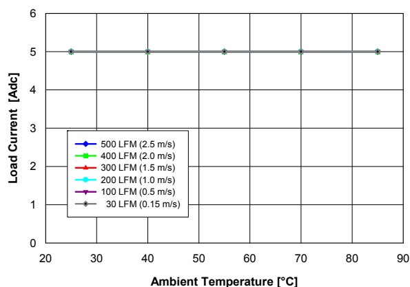
Fig. 1.8V.2: Available load current vs. ambient temperature and airflow rates for V_{out} = 1.8 V converter mounted horizontally with V_{in} = 5 V, air flowing from pin 5 to pin 1 and maximum MOSFET temperature \leq 120 °C.
