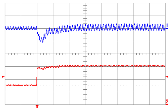
Fig. 1.2V.7: Output voltage response for V_{out} = 1.2 V to positive load current step change from 2.5 A to 5 A with slew rate of 5 A/ \mu s at V_{in} = 5 V. Top trace: output voltage (100 mV/div.); Bottom trace: load current (2 A/div.). C_o = 47 \mu F ceramic + 1 \mu F ceramic. Time scale: 20 \mu s/div.
