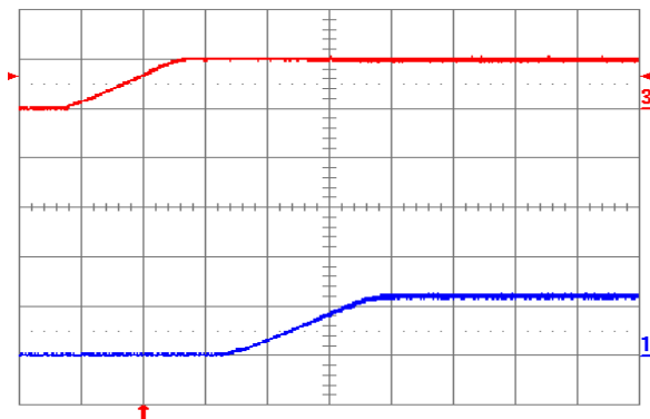
Fig. 1.2V.5: Turn-on transient for V_{out} = 1.2 V with application of V_{in} at full rated load current (resistive) and 47 \mu F external capacitance at V_{in} = 5 V. Top trace: V_{in} (5 V/div.); Bottom trace: output voltage (1 V/div.); Time scale: 2 ms/div.
