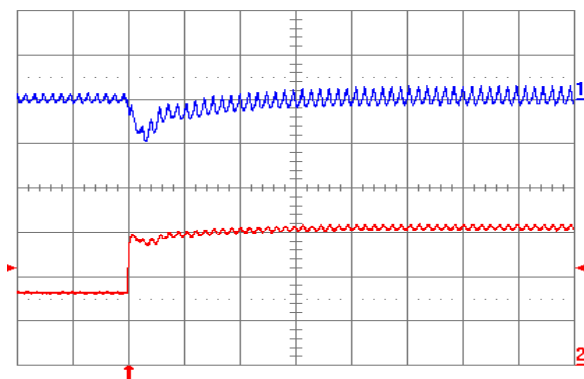
Fig. 0.7525V.7: Output voltage response for V_{out} = 0.7525 V to positive load current step change from 2.5 A to 5 A with slew rate of 5 A/ \mu s at V_{in} = 5 V. Top trace: output voltage (100 mV/div.); Bottom trace: load current (2 A/div.). C_o = 47 \mu F ceramic + 1 \mu F ceramic. Time scale: 20 \mu s/div.
