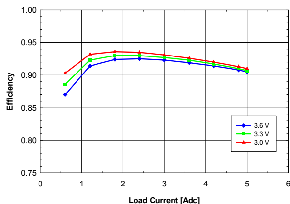
Fig. 1.8V.4: Efficiency vs. load current and input voltage for V_{out} = 1.8 V converter mounted vertically with air flowing from pin 5 to pin 1 at a rate of 200 LFM (1 m/s) and T_a = 25 °C.
