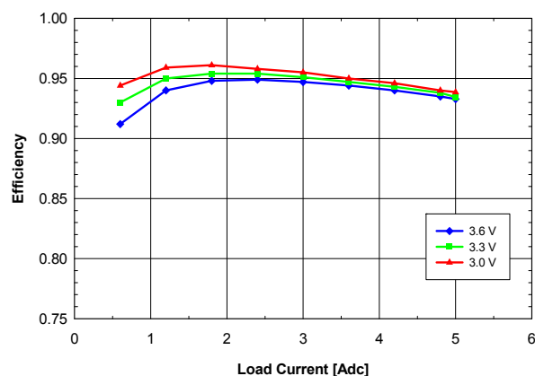
Fig. 2.5V.4: Efficiency vs. load current and input voltage for V_{out} = 2.5 V converter mounted horizontally with air flowing from pin 5 to pin 1 at a rate of 200 LFM (1 m/s) and T_a = 25 °C.
