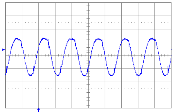
Fig. 2.5V.5: Output voltage ripple (20 mV/div.) at full rated load current into a resistive load with external capacitance 10 \mu F ceramic + 1 \mu F ceramic and V_{in} = 5 V for V_{out} = 2.5 V. Time scale: 2 \mu s/div.
