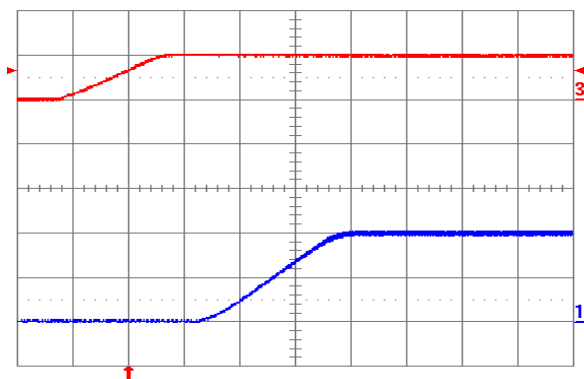
Fig. 2.0V.5: Turn-on transient for V_{out} = 2.0 V with application of V_{in} at full rated load current (resistive) and 47 \mu F external capacitance at V_{in} = 5 V. Top trace: V_{in} (5 V/div.); Bottom trace: output voltage (1 V/div.); Time scale: 2 ms/div.
