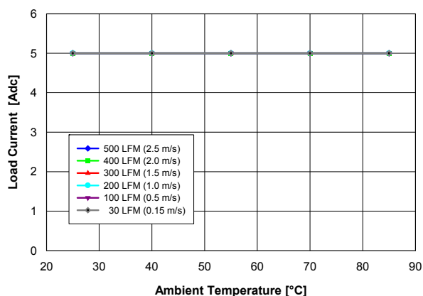
Fig. 3.3V.2: Available load current vs. ambient temperature and airflow rates for V_{out} = 3.3 V converter mounted horizontally with V_{in} = 5 V, air flowing from pin 5 to pin 1 and maximum MOSFET temperature \leq 120 °C.
