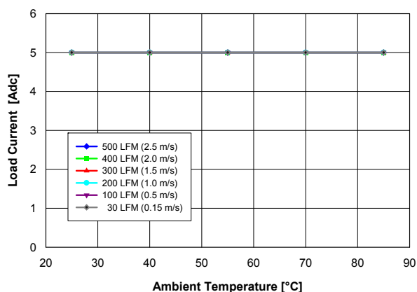
Fig. 0.7525V.1: Available load current vs. ambient temperature and airflow rates for V_{out} = 0.7525 V converter mounted vertically with V_{in} = 5 V, air flowing from pin 5 to pin 1 and maximum MOSFET temperature \leq 120 °C.
