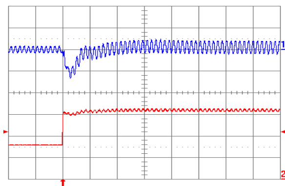
Fig. 2.0V.7: Output voltage response for V_{out} = 2.0 V to positive load current step change from 2.5 A to 5 A with slew rate of 5 A/ \mu s at V_{in} = 5 V. Top trace: output voltage (100 mV/div.); Bottom trace: load current (2 A/div.). C_o = 47 \mu F ceramic + 1 \mu F ceramic. Time scale: 20 \mu s/div.
