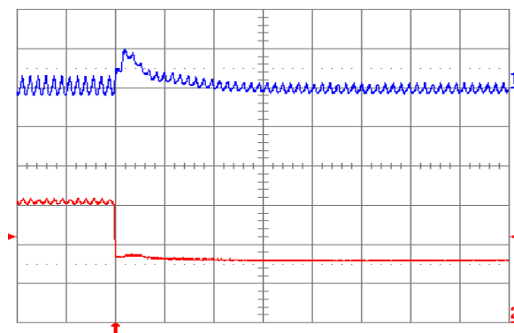
Fig. 1.0V.8: Output voltage response for V_{out} = 1.0 V to negative load current step change from 5 A to 2.5 A with slew rate of -5 A/ \mu s at V_{in} = 5 V. Top trace: output voltage (100 mV/div.); Bottom trace: load current (2 A/div.). C_o = 47 \mu F ceramic + 1 \mu F ceramic. Time scale: 20 \mu s/div.
