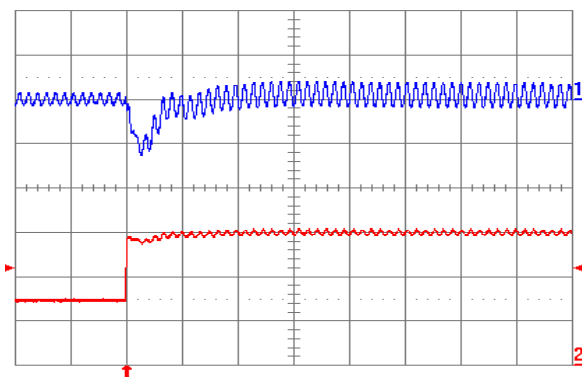
Fig. 1.8V.7: Output voltage response for V_{out} = 1.8 \text{ V} to positive load current step change from 2.5 A to 5 A with slew rate of 5 \text{ A}/\mu\text{s} at V_{in} = 5 \text{ V} . Top trace: output voltage (100 mV/div.); Bottom trace: load current (2 A/div.). C_o = 47 \mu\text{F} ceramic + 1 \mu\text{F} ceramic. Time scale: 20 \mu\text{s} /div.
