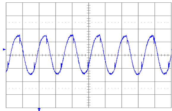
Fig. 2.0V.6: Output voltage ripple (20 mV/div.) at full rated load current into a resistive load with external capacitance 10 \mu F ceramic + 1 \mu F ceramic and V_{in} = 5 V for V_{out} = 2.0 V. Time scale: 2 \mu s/div.
