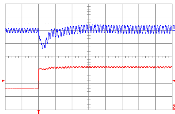
Fig. 2.5V.7: Output voltage response for V_{out} = 2.5 V to positive load current step change from 2.5 A to 5 A with slew rate of 5 A/ \mu s at V_{in} = 5 V. Top trace: output voltage (100 mV/div.); Bottom trace: load current (2 A/div.). C_o = 47 \mu F ceramic + 1 \mu F ceramic. Time scale: 20 \mu s/div.
