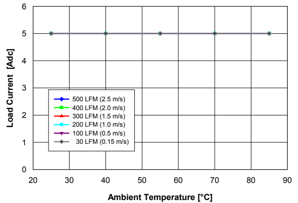
Fig. 2.0V.2: Available load current vs. ambient temperature and airflow rates for V_{out} = 2.0 V converter mounted horizontally with V_{in} = 5 V, air flowing from pin 5 to pin 1 and maximum MOSFET temperature \leq 120 °C.
