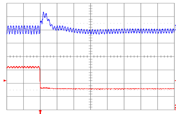
Fig. 2.5V.8: Output voltage response for V_{out} = 2.5 V to negative load current step change from 5 A to 2.5 A with slew rate of -5 A/ \mu s at V_{in} = 5 V. Top trace: output voltage (100 mV/div.); Bottom trace: load current (2 A/div.). C_o = 47 \mu F ceramic + 1 \mu F ceramic. Time scale: 20 \mu s/div.
