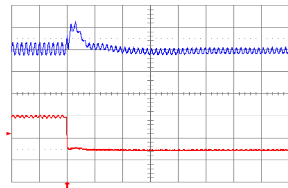
Fig. 1.8V.8: Output voltage response for V_{out} = 1.8 \text{ V} to negative load current step change from 5 A to 2.5 A with slew rate of -5 \text{ A}/\mu\text{s} at V_{in} = 5 \text{ V} . Top trace: output voltage (100 mV/div.); Bottom trace: load current (2 A/div.). C_o = 47 \mu\text{F} ceramic + 1 \mu\text{F} ceramic. Time scale: 20 \mu\text{s} /div.
