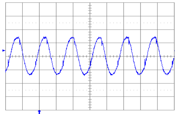
Fig. 1.8V.6: Output voltage ripple (20 mV/div.) at full rated load current into a resistive load with external capacitance 10 \mu\text{F} ceramic + 1 \mu\text{F} ceramic and V_{in} = 5 \text{ V} for V_{out} = 1.8 \text{ V} . Time scale: 2 \mu\text{s} /div.
