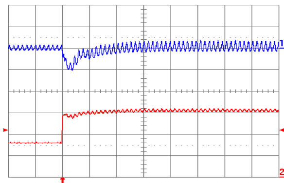
Fig. 1.0V.7: Output voltage response for V_{out} = 1.0 V to positive load current step change from 2.5 A to 5 A with slew rate of 5 A/ \mu s at V_{in} = 5 V. Top trace: output voltage (100 mV/div.); Bottom trace: load current (2 A/div.). C_o = 47 \mu F ceramic + 1 \mu F ceramic. Time scale: 20 \mu s/div.
