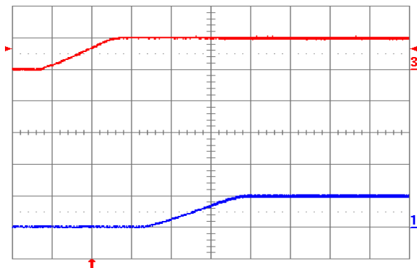
Fig. 1.0V.5: Turn-on transient for V_{out} = 1.0 V with application of V_{in} at full rated load current (resistive) and 47 \mu F external capacitance at V_{in} = 5 V. Top trace: V_{in} (5 V/div.); Bottom trace: output voltage (1 V/div.); Time scale: 2 ms/div.
