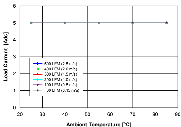
Fig. 1.5V.2: Available load current vs. ambient temperature and airflow rates for V_{out} = 1.5 V converter mounted horizontally with V_{in} = 5 V, air flowing from pin 5 to pin 1 and maximum MOSFET temperature \leq 120 °C.
