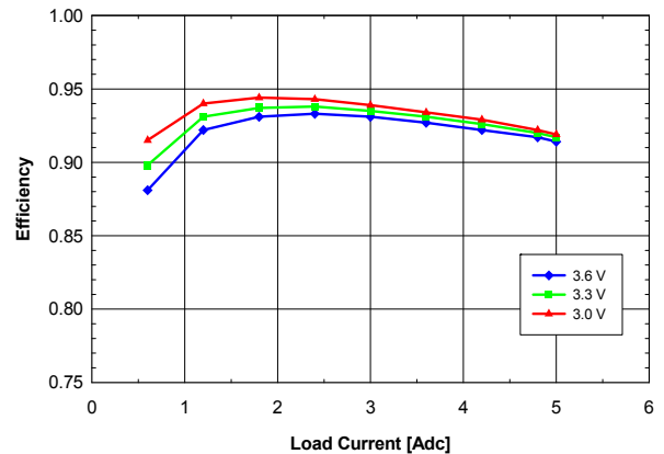
Fig. 2.0V.4: Efficiency vs. load current and input voltage for V_{out} = 2.0 V converter mounted horizontally with air flowing from pin 5 to pin 1 at a rate of 200 LFM (1 m/s) and T_a = 25 °C.
