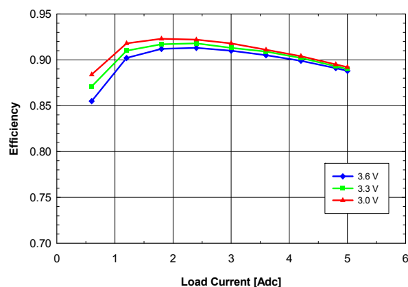
Fig. 1.5V.4: Efficiency vs. load current and input voltage for V_{out} = 1.5 V converter mounted horizontally with air flowing from pin 5 to pin 1 at a rate of 200 LFM (1 m/s) and T_a = 25 °C.
