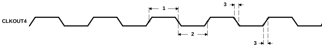
Figure 5-12. CLKOUT4 Timing
