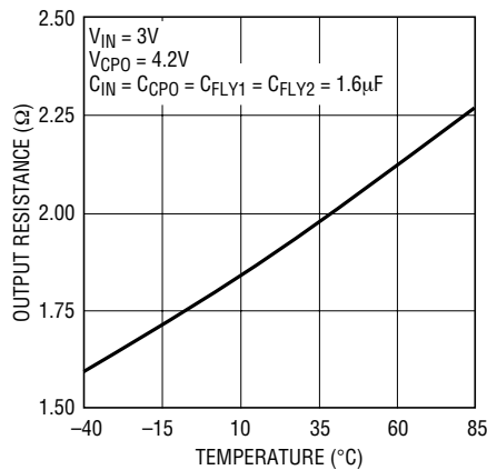
1.5x Mode Charge Pump Open-Loop Output Resistance vs Temperature ( 1.5V_{IN} - V_{CPO} )/ICP0
