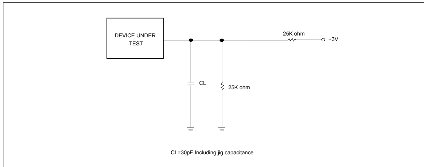
Figure 87. OUTPUT LOADING
