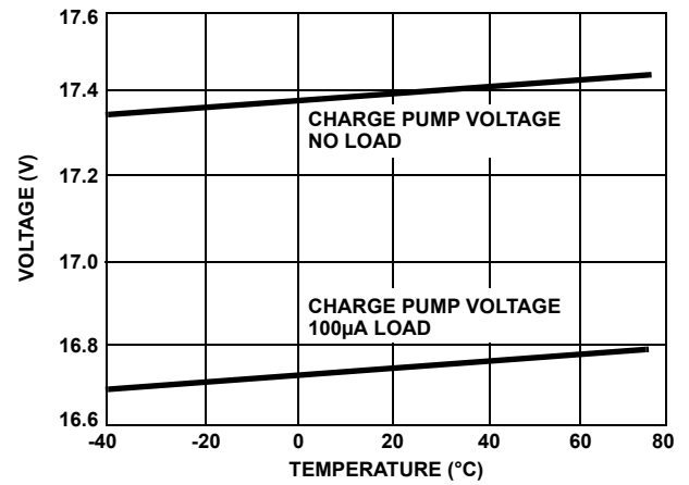
FIGURE 9. PUMP VOLTAGE
