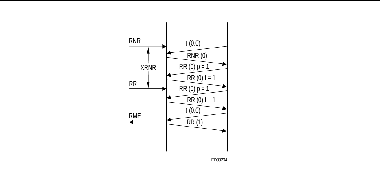
Figure 13 Flow Control/Reception
