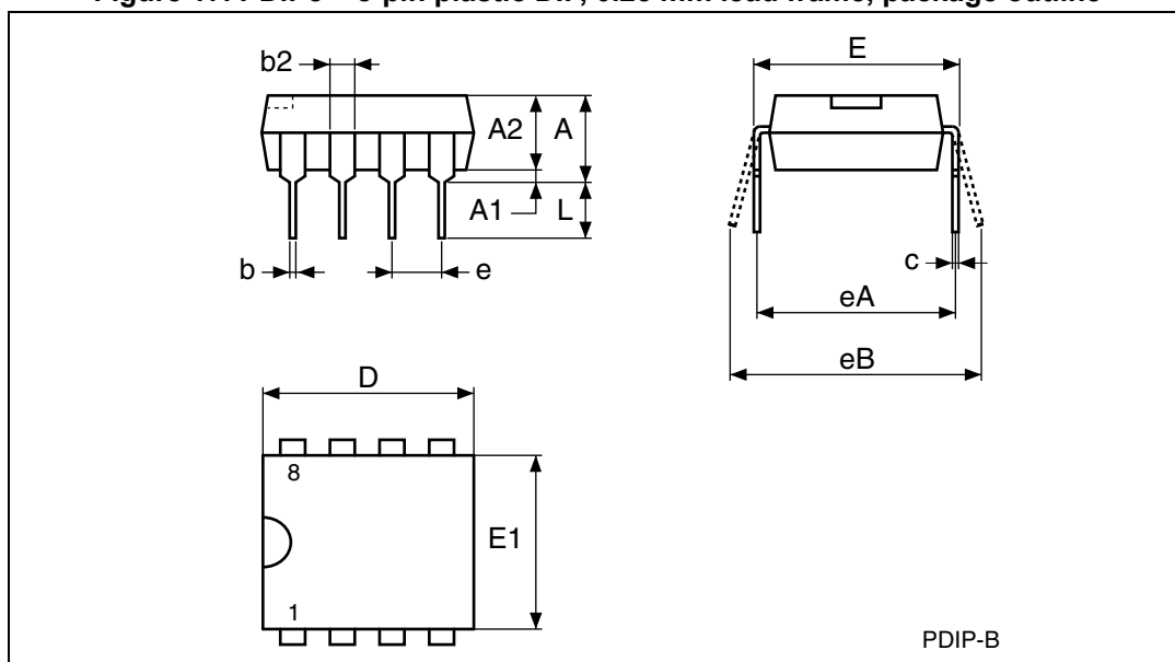
Figure 17. PDIP8 – 8-pin plastic DIP, 0.25 mm lead frame, package outline
