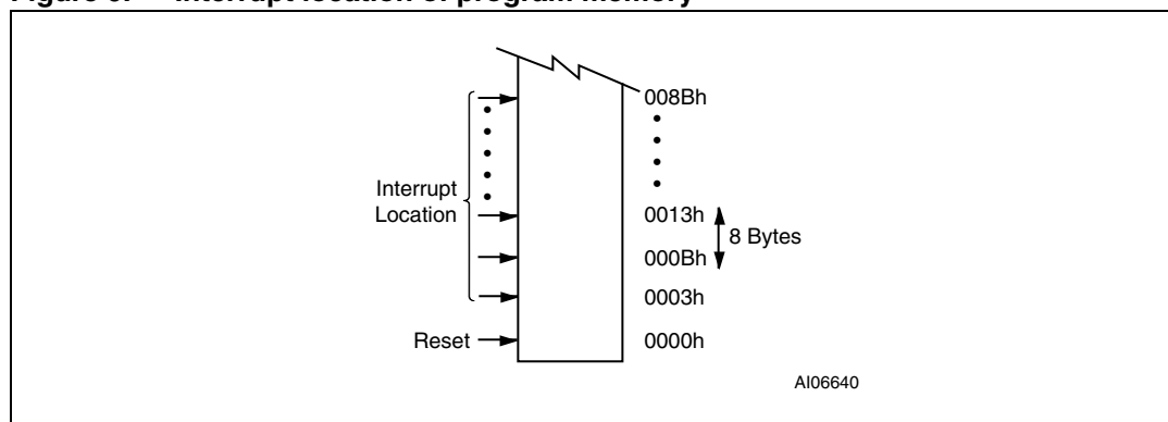
Figure 9. Interrupt location of program memory
