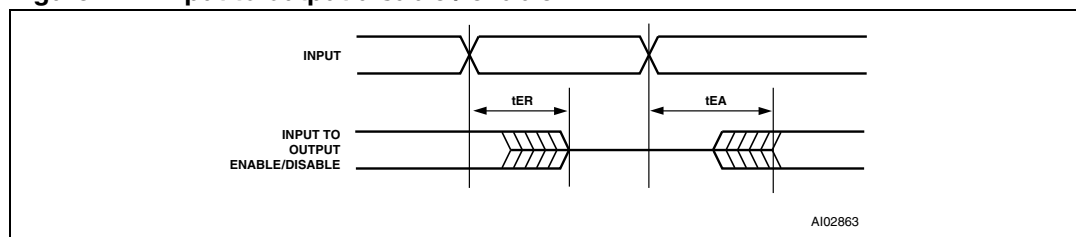
Figure 72. Input to output disable / enable
