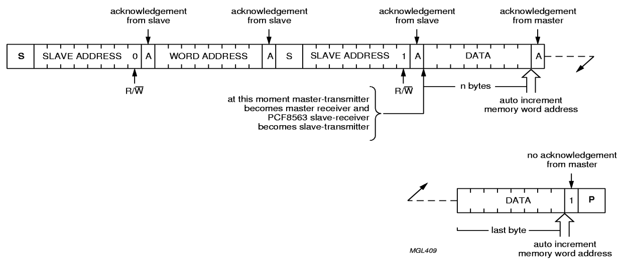
Fig.10 Master reads after setting word address (write word address; READ data).
