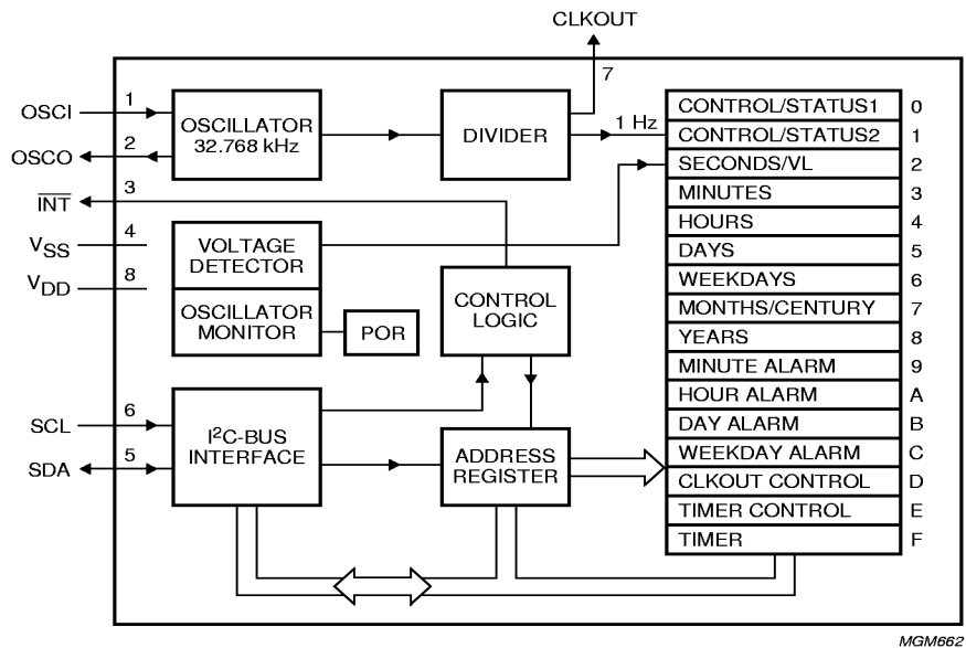
Fig.1 Block diagram PCF8563 real-time clock/calendar.
