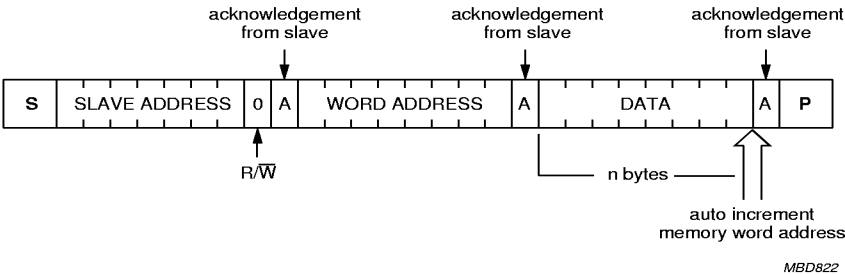
Fig.9 Master transmits to slave receiver (WRITE) mode.
