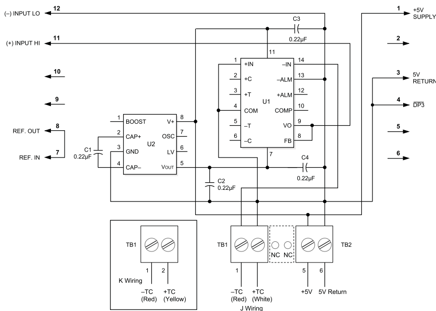
Figure 1. DMS-EB-TCJ/TCK Schematic Diagram
