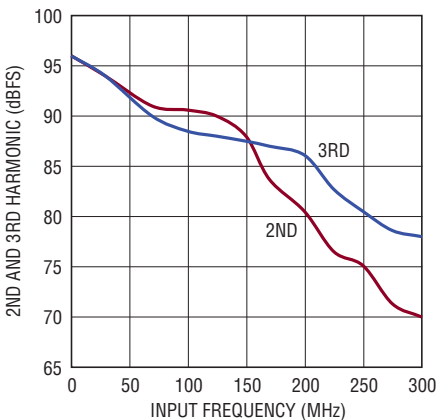
LTC2181: 2nd, 3rd Harmonic vs Input Frequency, -1\text{dBFS} , 40\text{Mps} , 2\text{V} Range
