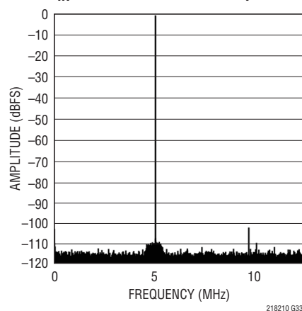
LTC2180: 64k Point FFT, f_{IN} = 5\text{MHz} , -1dBFS, 25MSPS
