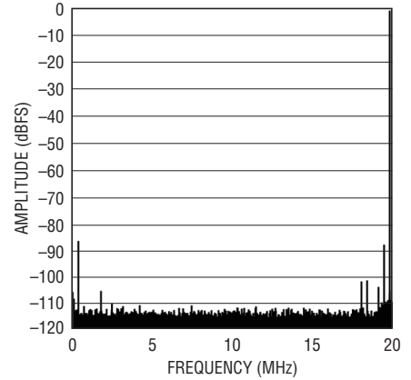
LTC2181: 64k Point FFT, f_{IN} = 140\text{MHz} , -1\text{dBFS} , 40\text{Mps}
