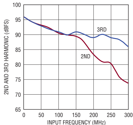
LTC2181: 2nd, 3rd Harmonic vs Input Frequency, -1\text{dBFS} , 40\text{Mps} , 1\text{V} Range
