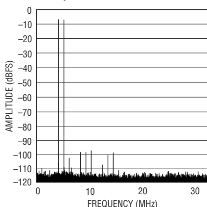
LTC2182: 64k Point 2-Tone FFT, f_{IN} = 69\text{MHz} , 70MHz, -7dBFS, 65Msps
