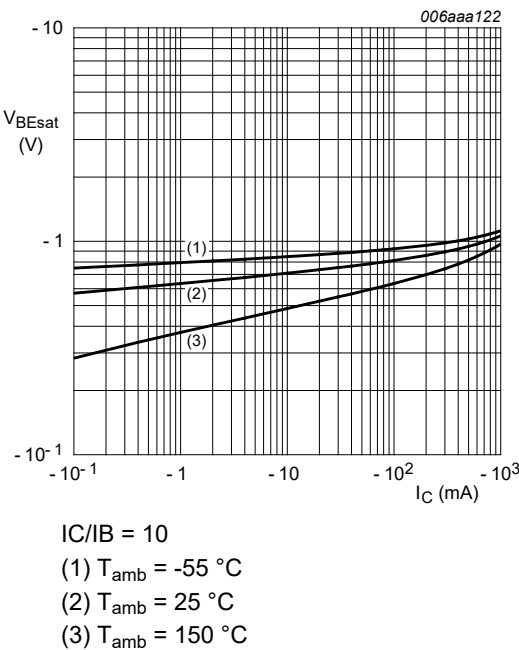
Fig. 5. BC807-16: Base-emitter saturation voltage as a function of collector current; typical values
