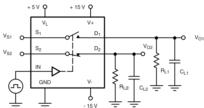
Figure 3. Break-Before-Make
