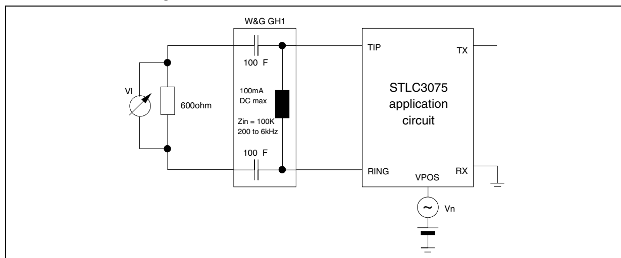
Figure 17. PSRR Power supply rejection V_{pos} to 2W port PSSRC = 20\text{Log}|V_n/V_I|
