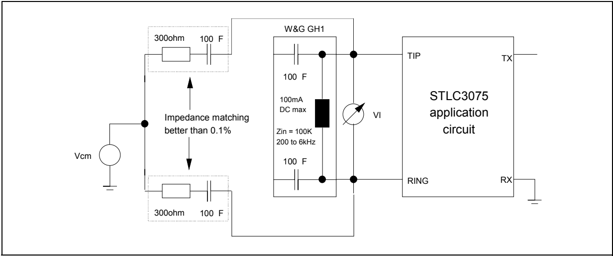
Figure 19. T/L Transversal to Longitudinal Conversion T/L = 20\text{Log}|V_{rx}/V_{cm}|
