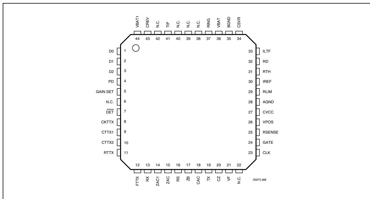
Figure 3. Pin Connection
