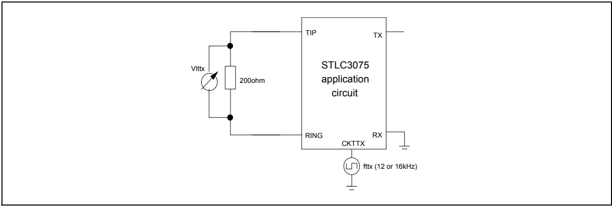
Figure 20. VTXX Metering Pulse level on line
