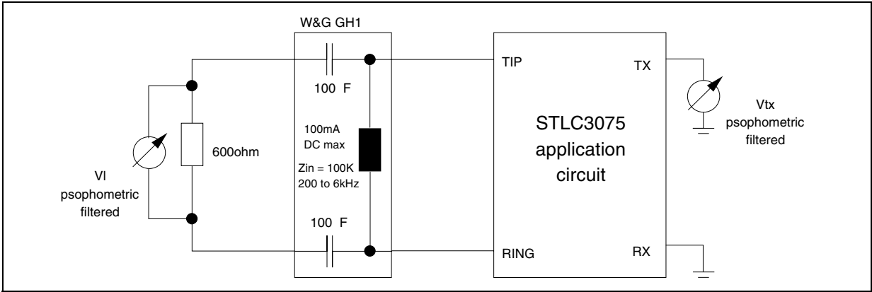
Figure 21. V2Wp and W4Wp: Idle channel psophometric noise at line and TX. V2Wp = 20\text{Log}|V_I/0.774I| ; V4Wp = 20\text{Log}|V_{tx}/0.774I|
