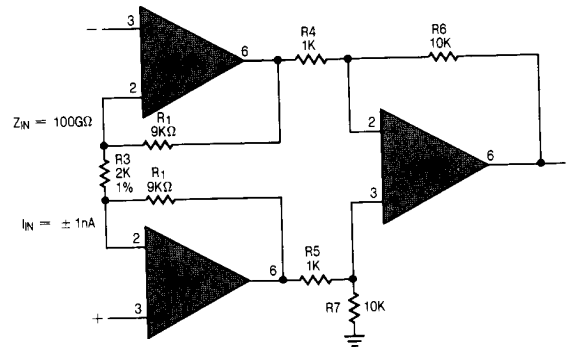
Instrumentation Amplifier
