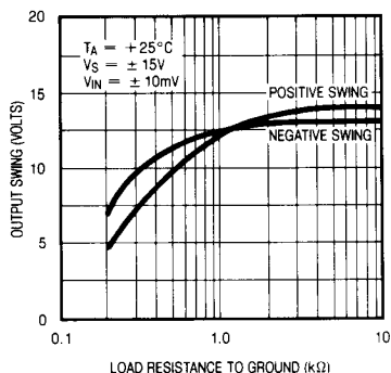
Output Voltage vs Load Resistance
