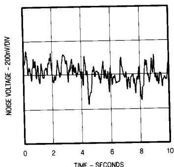
Low Frequency Noise (Closed Loop Gain = 25,000)
