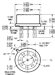
H Package Metal Can
