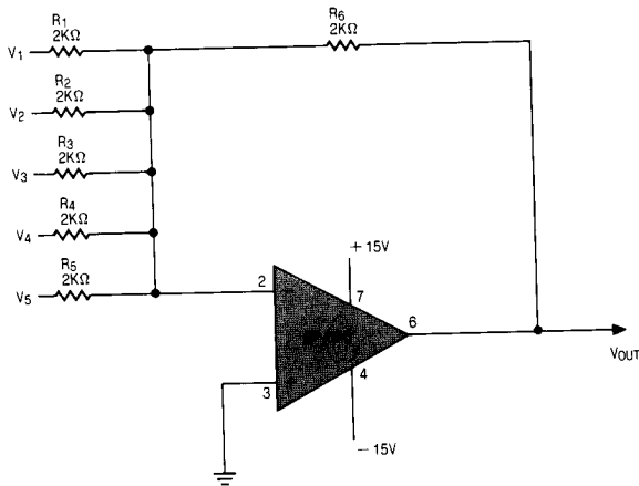
Precision Summing Amplifier
