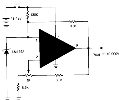
Precision Buffered Single Supply Reference
