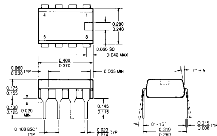
N8 Package 8 Lead Plastic
