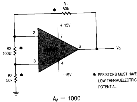
Offset Voltage Test Circuit †
