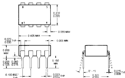
J8 Package 8 Lead Hermetic Dip
