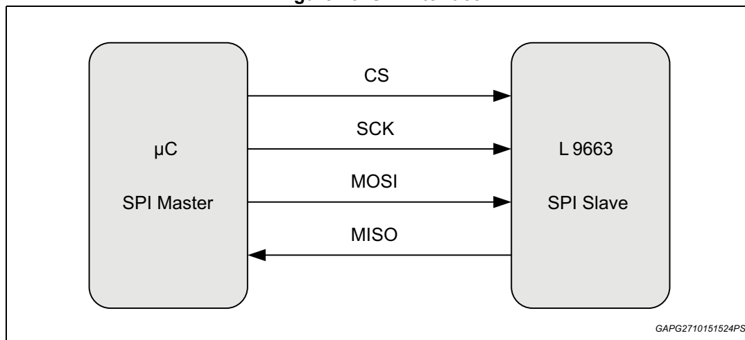
Figure 26. SPI interface
