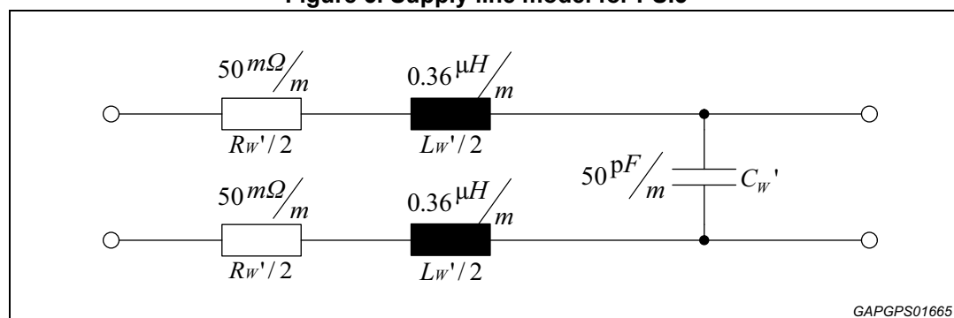
Figure 5. Supply line model for PSI5
