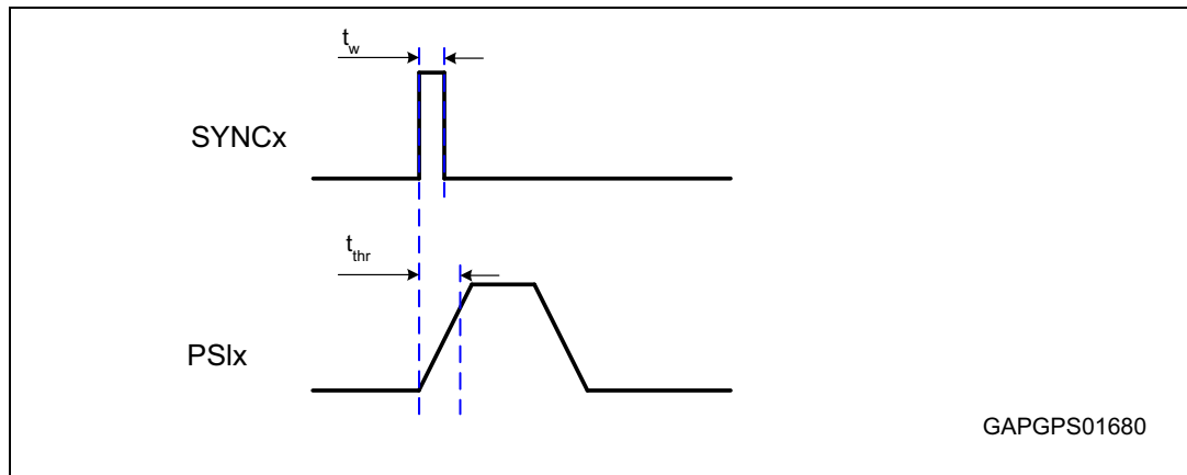
Figure 21. Short (in case 1\mu\text{s} < t_w < 5\mu\text{s} ) Sync Pulse trigger, compliant to PSI5 standard
