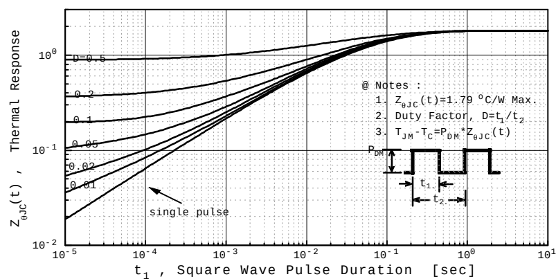
Fig 11. Thermal Response
